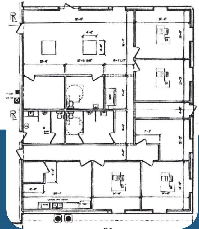
Office Plan
