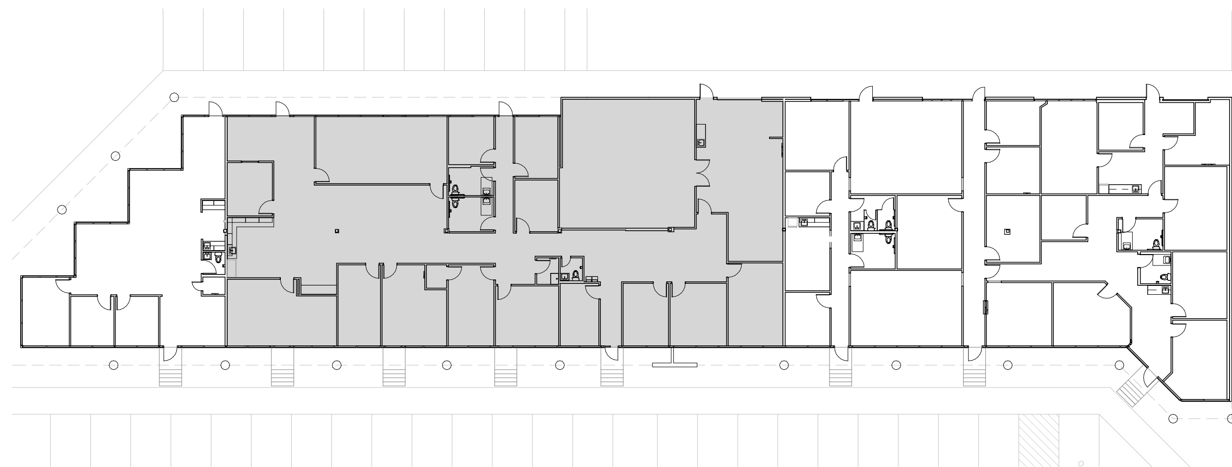
② Key Plan - 4808-4934 3/64" = 1'-0"
