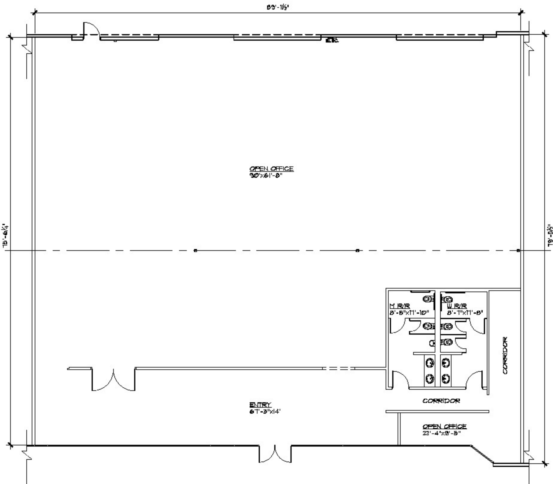
01 AS-BUILT FLOOR PLAN SUITE 209 - SUITE 6,897 S.F. SCALE: GRAPHIC
