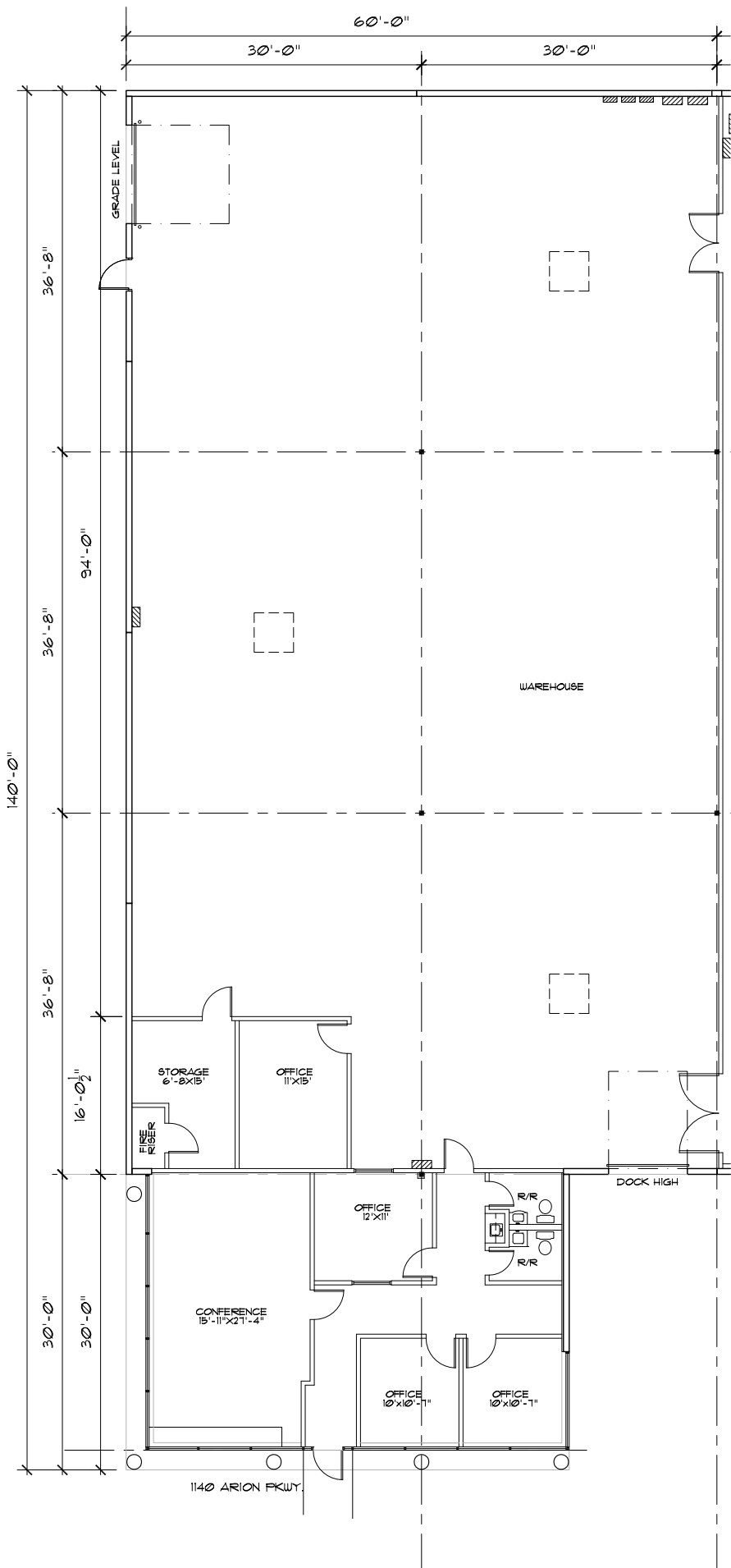
AS-BUILT FLOOR PLAN-7,950 S.F. SCALE: 1/16" = 1'-0"
