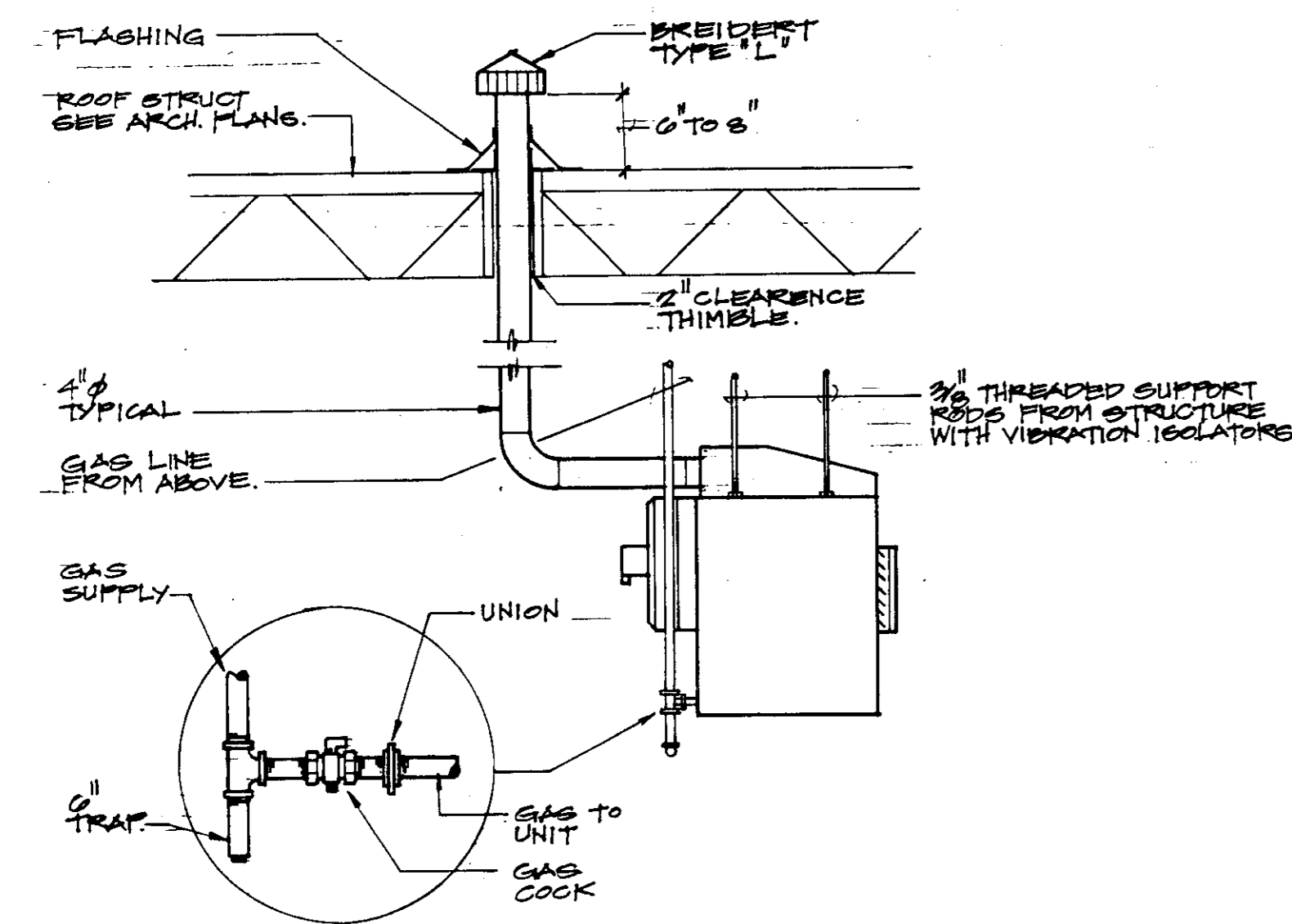
102 UNIT HEATER DETAIL NO SCALE
