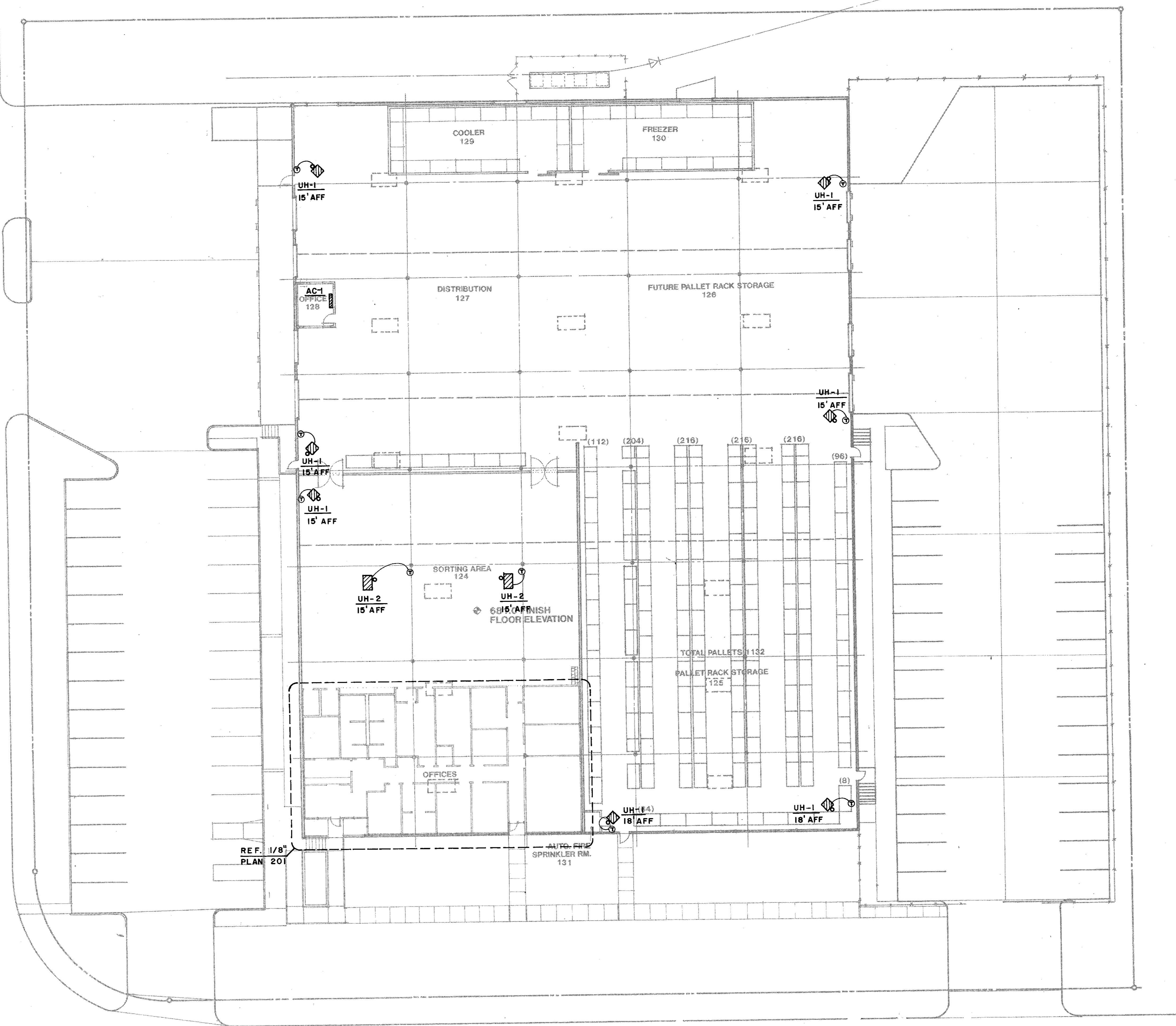
101 HVAC FLOOR PLAN SCALE: 1/16" = 1'-0"
